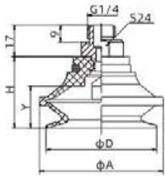
SZB50□-G2M
