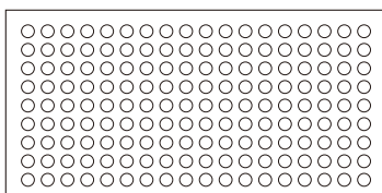
EGP200 standardised suction-hole type Type: P20 Universal type
