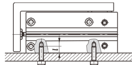
Vertical Mounting (Tapped Holes)
