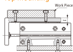
Top Mounting
