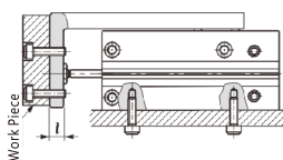
Top Mounting
