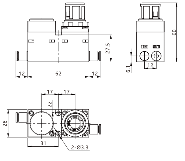
ERM1000F-4-□
