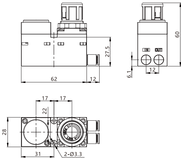
ERM1000F-1-□
