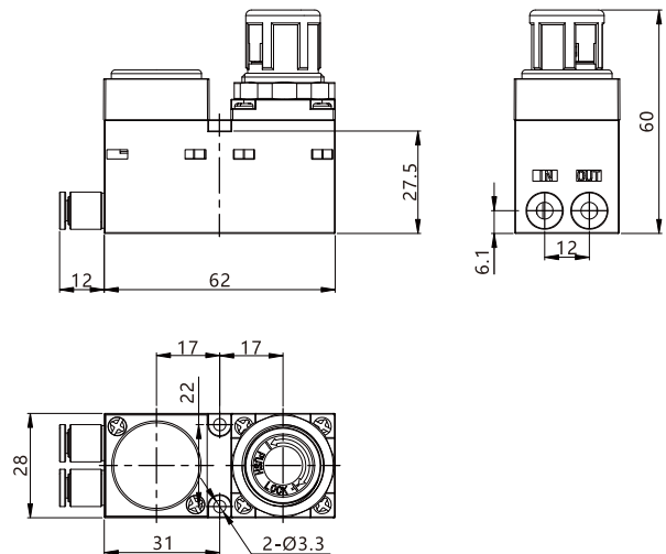
ERM1000F-2-□
