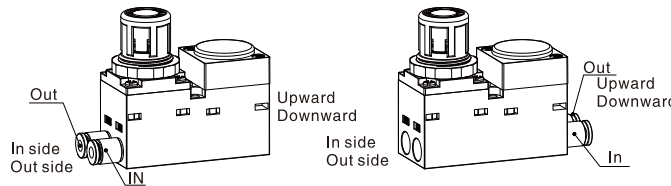
Piping Direction Diagram
